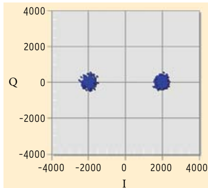
FIGURE 3 GLONASS BPSK signal after code and carrier synchronization and \tau second accumulation (actual \tau second accumulator outputs of a GNSS receiver).
