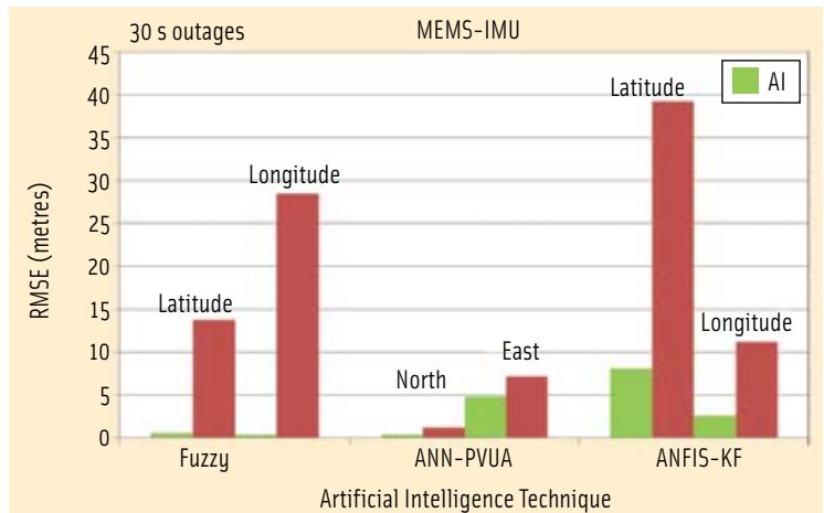
FIGURE 4 MEMS-based IMU comparison chart
