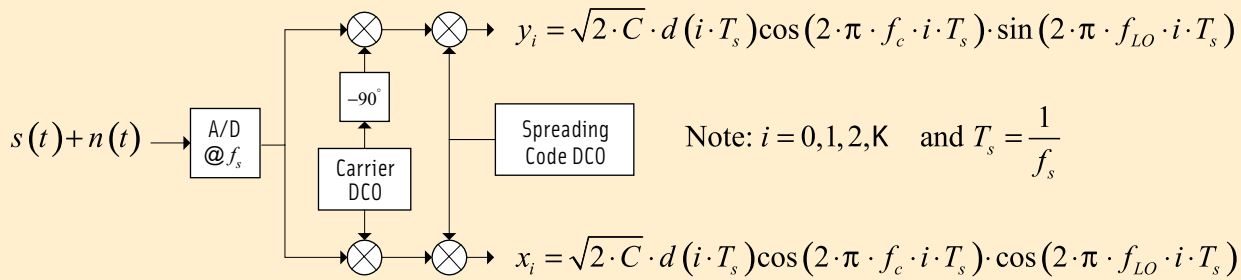
FIGURE 2 Carrier power estimation (spreading code synchronized)
