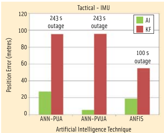
FIGURE 3 Tactical IMU comparison chart
