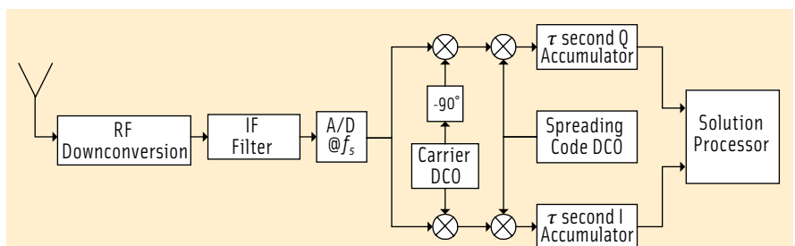
FIGURE 1 Typical GNSS receiver block diagram
