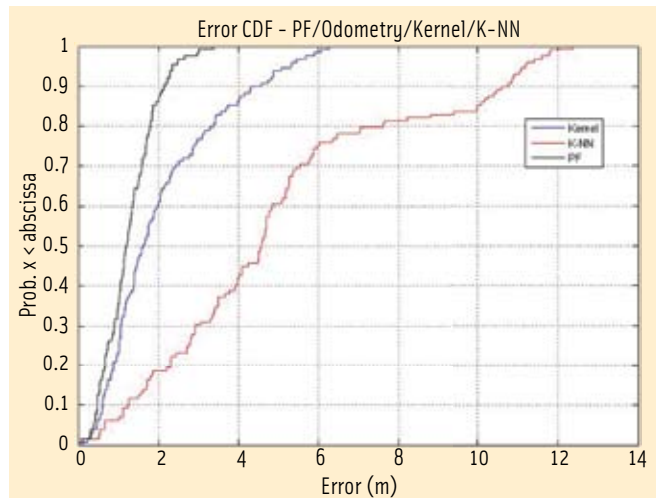
FIGURE 2 CDF of the localization error for two different Wi-Fi localization algorithms and a Particle Filter (PF) combining the results of Wi-Fi localization and an inertial system in the indoor route shown in Figure 3.
