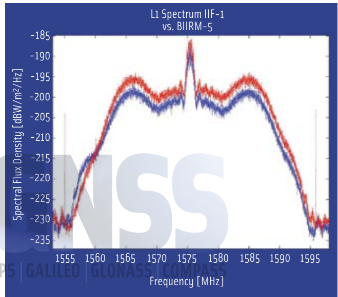
FIGURE 6 L1 Spectrum of IIF-1 (red) and BIIR-M5 (blue) recorded at 80° elevation angle
