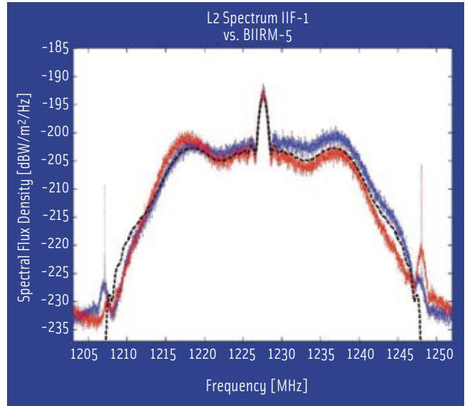
FIGURE 8 L2 Spectrum of IIF-1 (red) and BIIR-M5 (blue) recorded at 80° elevation angle
