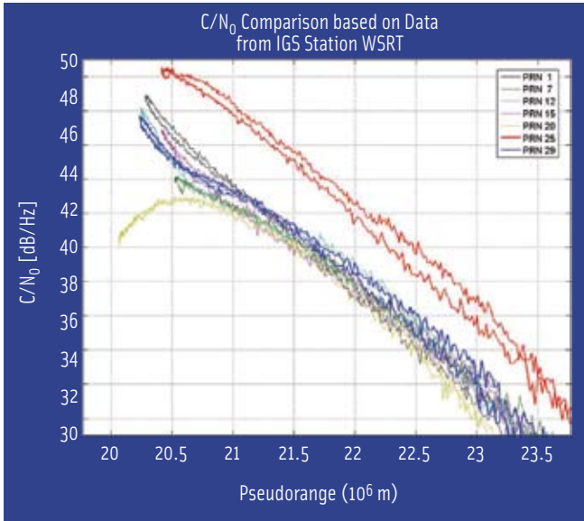
FIGURE 7 C/N 0 vs. Pseudorange comparison of several GPS satellites. IIF (PRN25) red and BIIR-M5 (PRN29) blue. Plot is based on the data captured on Day 170 (Jun 19).
